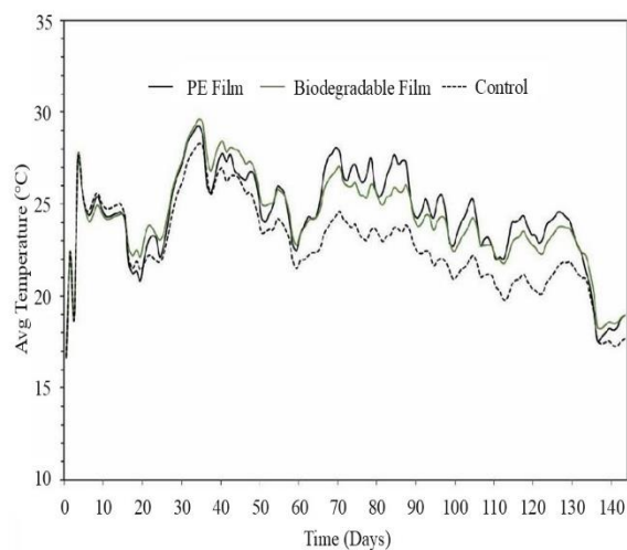
Figure 4. Changes in soil temperature in cotton fields with PE film, biodegradable film and with no film
