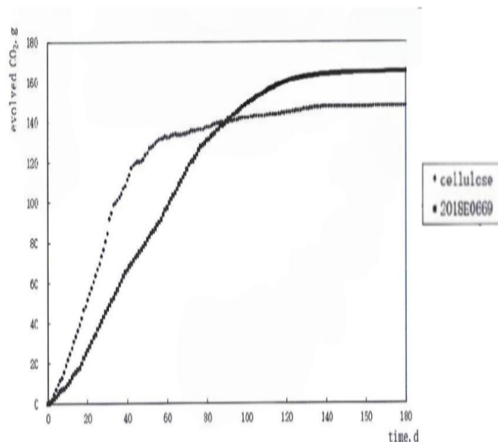
Figure 3. Curve of degree of biodegradation
