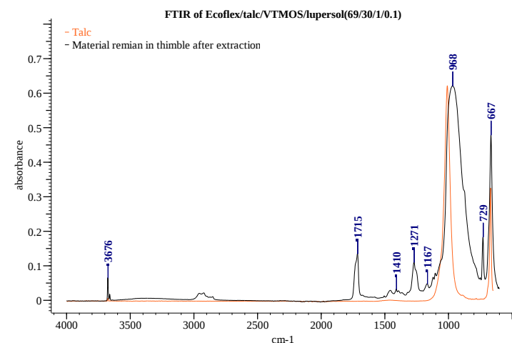
Figure 1. FTIR spectrum of Ecoflex/silane/Talc after extraction (in thimble) vs. Talc
